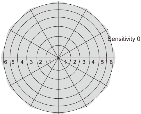
Ceiling Pattern (Unit: m) Installation Height: 10m
